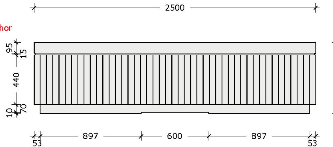
2 Front View Scale: 1 : 20
