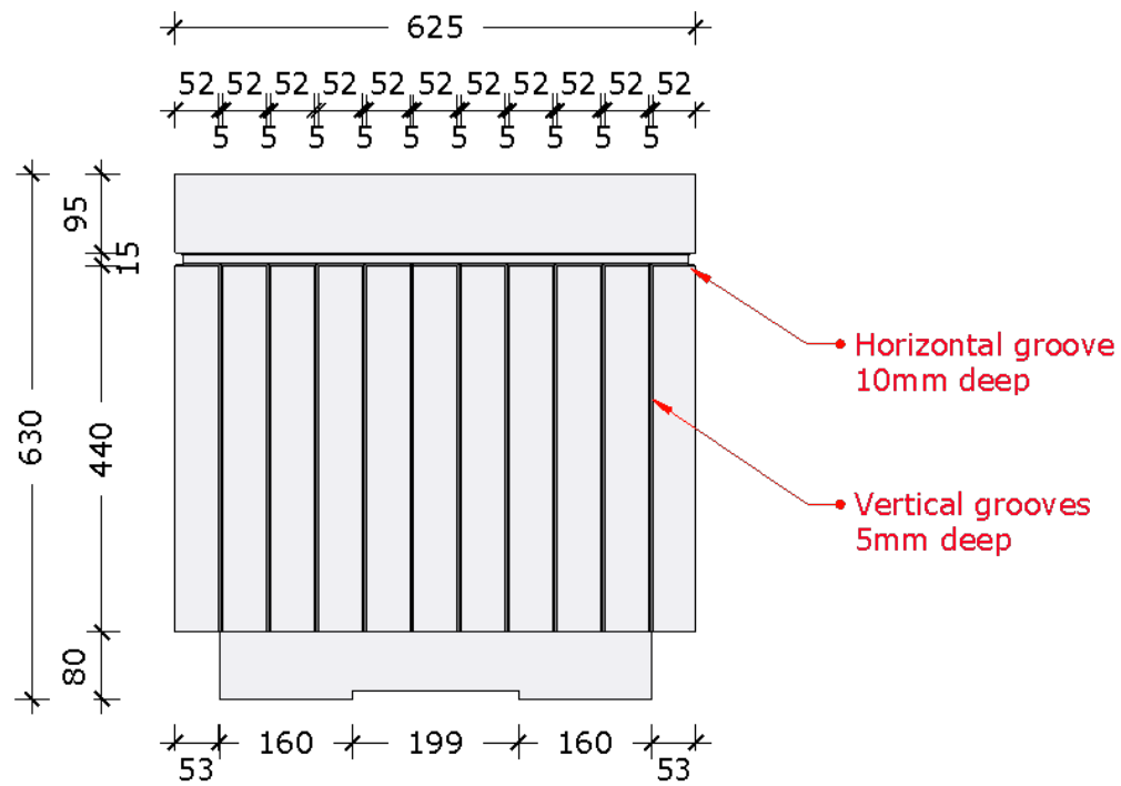
2 Typical Transverse Side Texture Scheme Scale: 1 : 10
