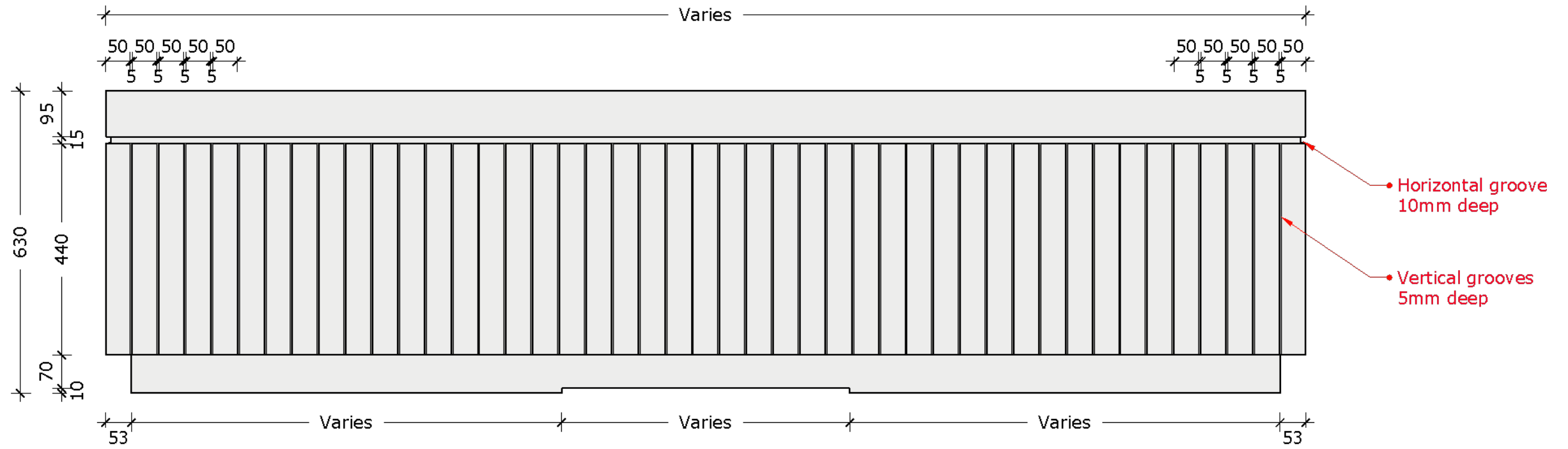
1 Typical Longitudinal Side Texture Scheme Scale: 1 : 10
