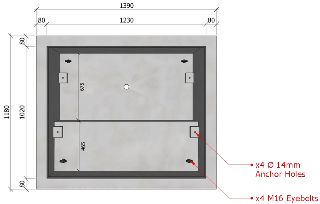
1 Plan View
