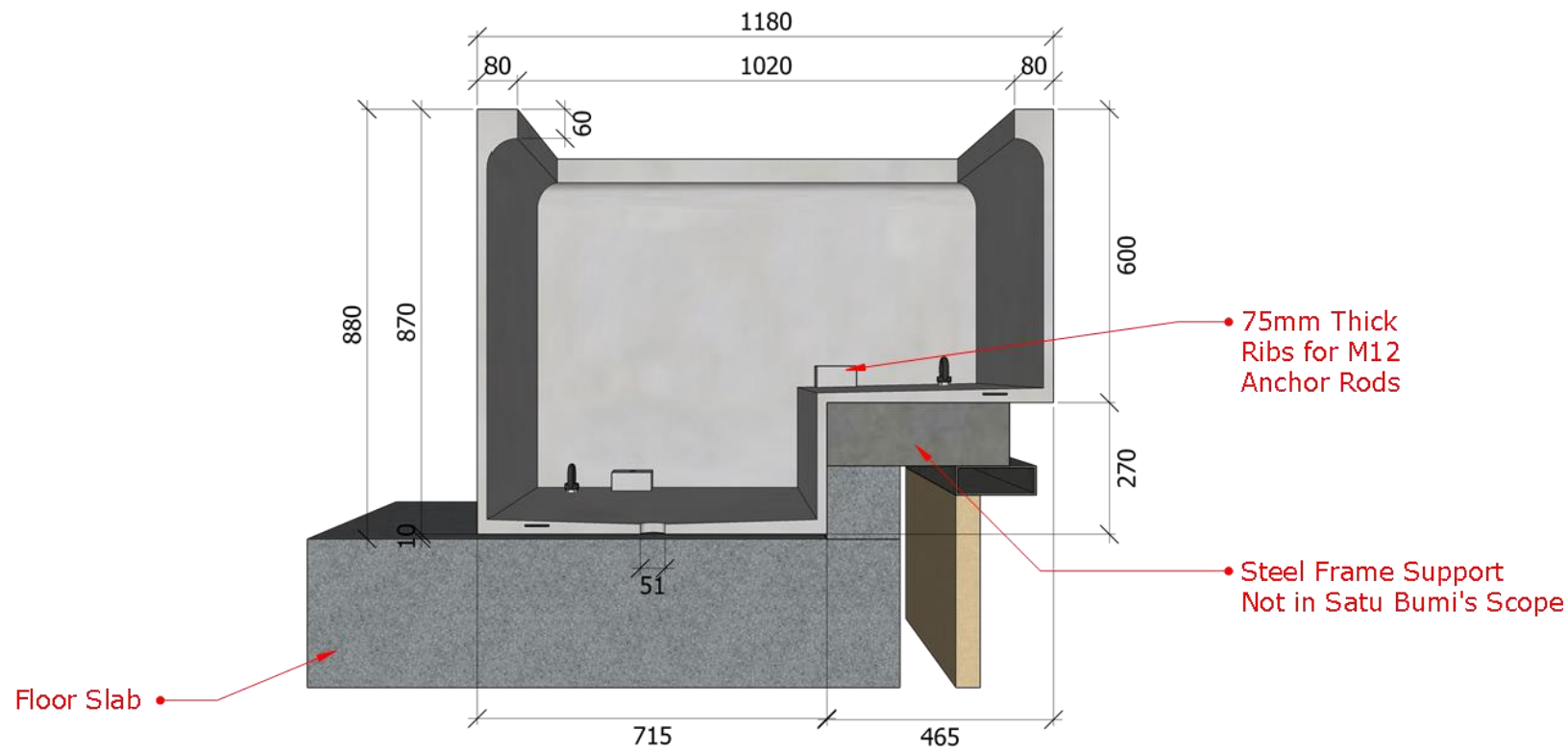
3 Section View
