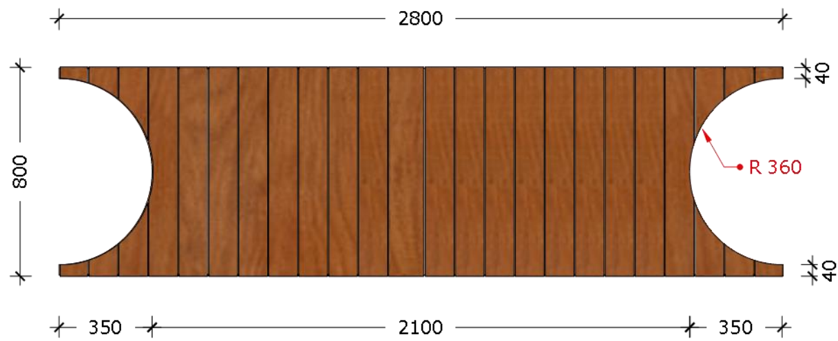
1 Plan View
