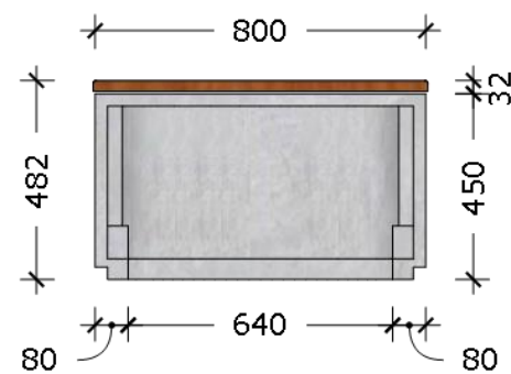
5 Cross Section
