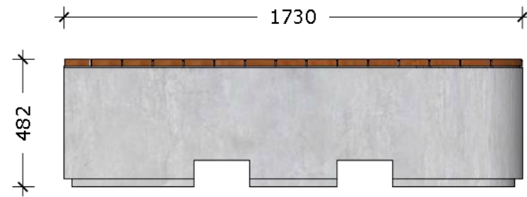
2 Front View
