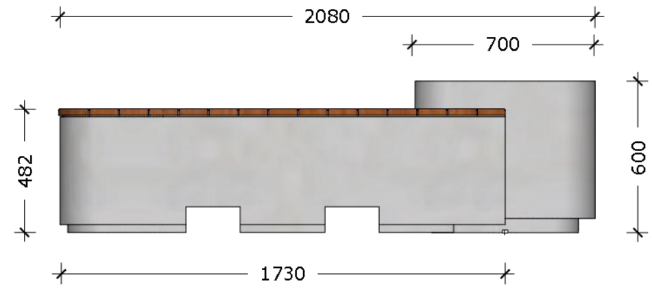
2 Front View
