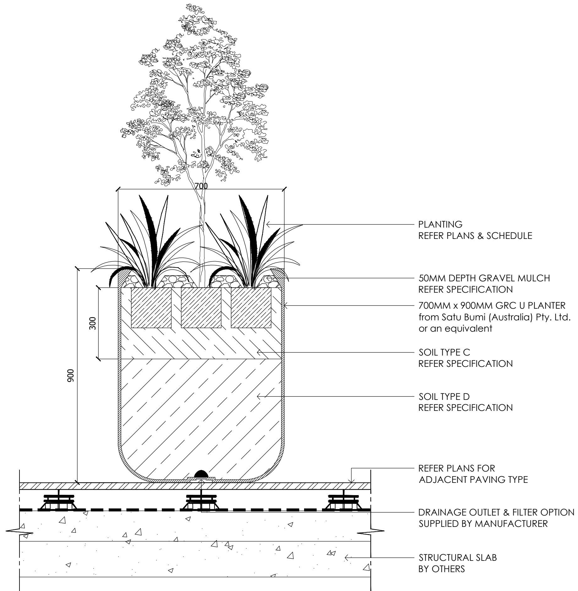
05 U PLANTER - TALL 700D x 900H 702 SCALE 1:10
